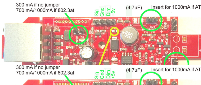
Internal jumpers and OEM options
