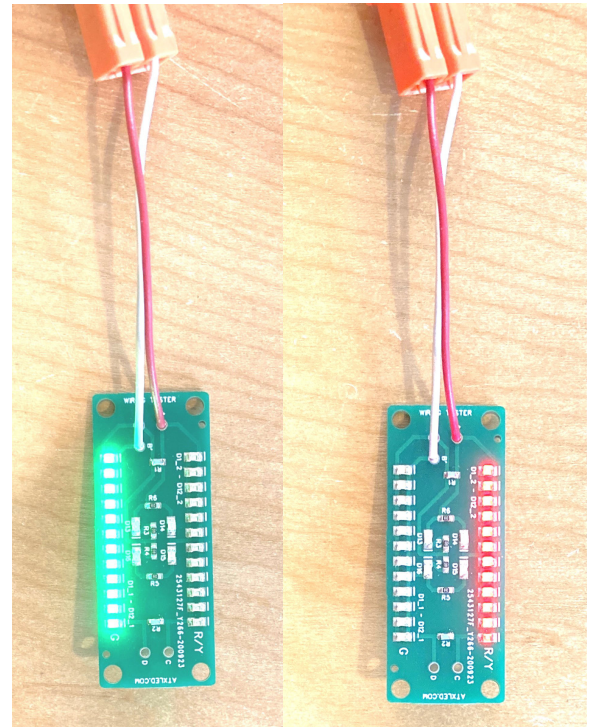
Proper Wiring
