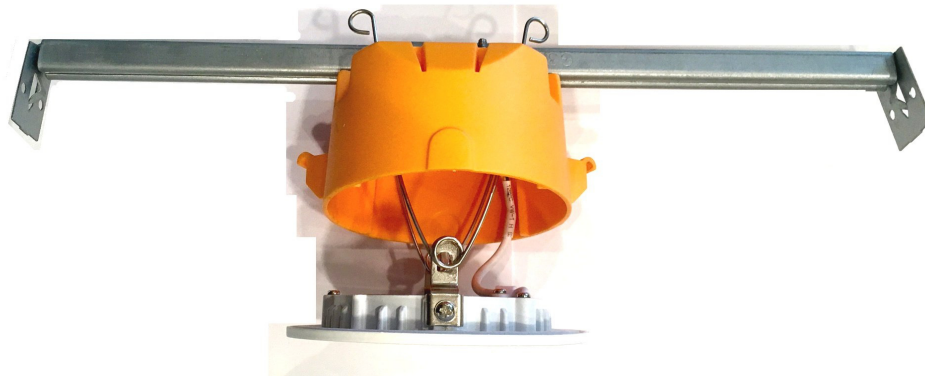
Screw-less mounting box for LEDs
