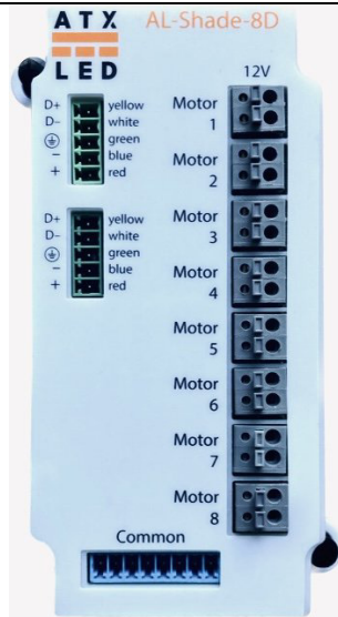
8 Channel Shade driver
